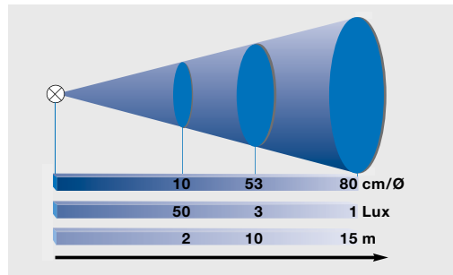
Range-diagram Stabex HF-LED
