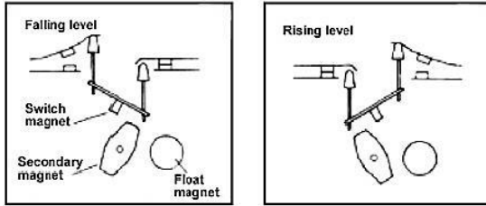
Schematic showing three-magnet system
