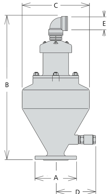
Flange Connection
