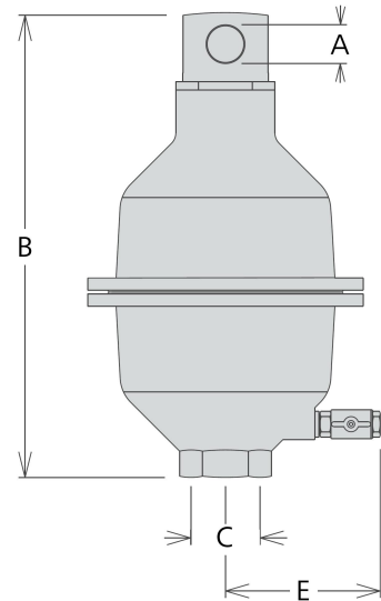
Sleeve Connection
