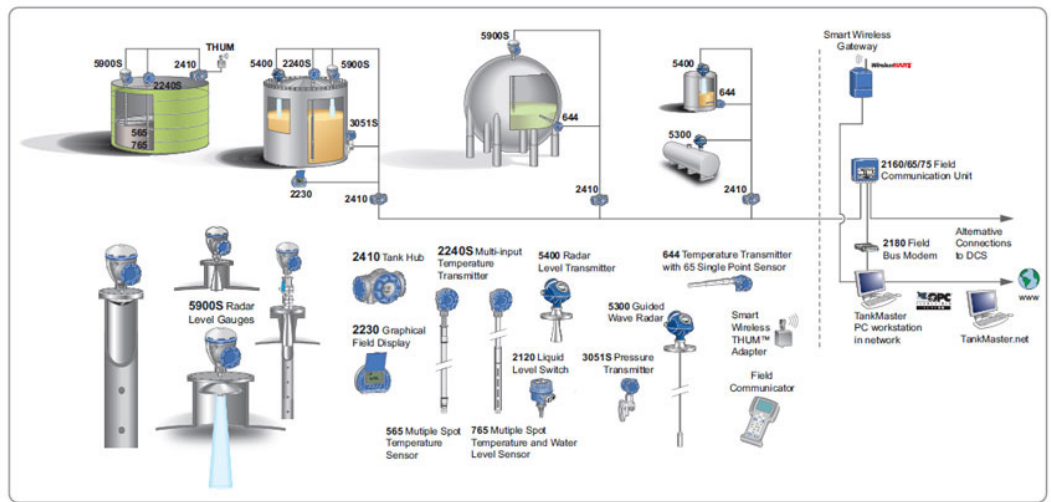
Wireless Rosemount Tank Gauging System
