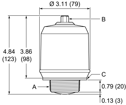
Figure 11: Rosemount 1208C
